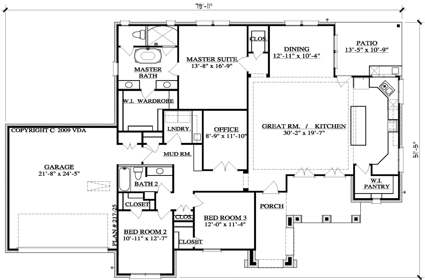
COPYRIGHT © 2009 VDA PLAN # 217-25 FLOOR LAYOUT
