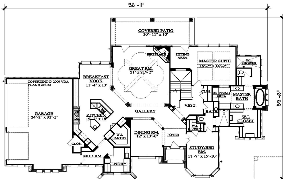
MAIN LEVEL FLOOR LAYOUT
